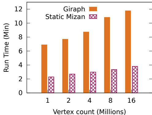
Figure 12. Comparing Mizan vs. Giraph using PageRank on regular random graphs, the graphs are uniformly distributed with each has around 17M edge
