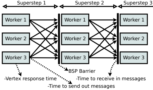
Figure 1. Factors that can affect the runtime in the Pregel framework
