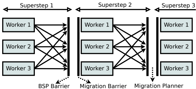
Figure 5. Mizan's BSP flow with migration planning
